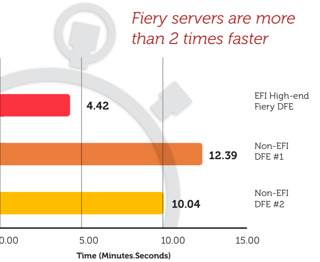
RIP and hold time: 576-page, 3.5 GB PDF file
